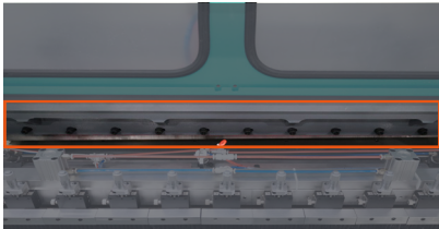
定长裁切机构 Preset Length Cutting Mechanism
