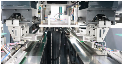
折边机构 Edge Folding Mechanism
