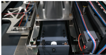
压料装置 Towel Pressing Mechanism
